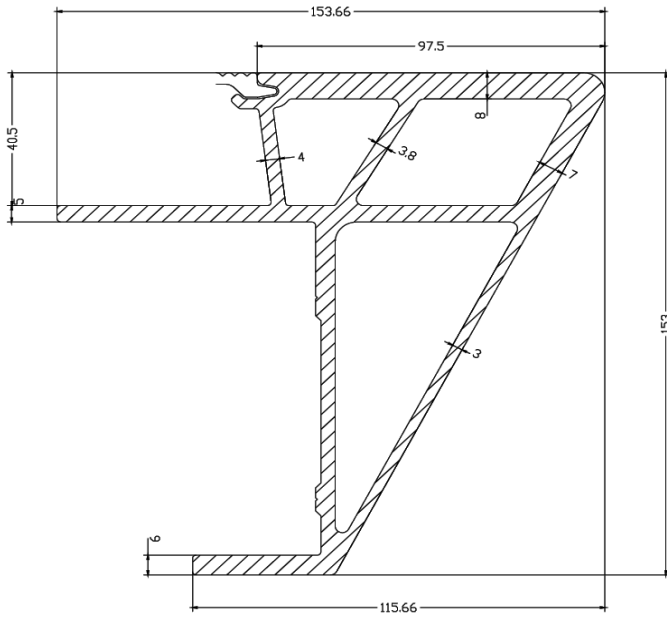
ATP112 8.298 kg/m
