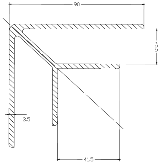
ATP140 2.802 kg/m
