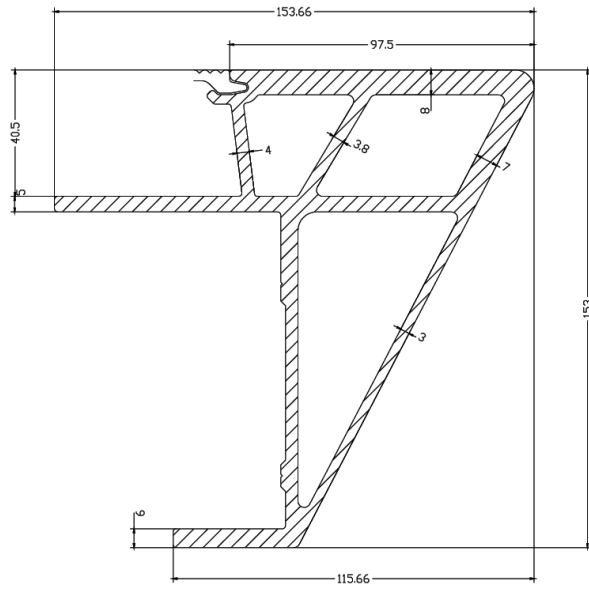
ATP112 8.298 kg/m
